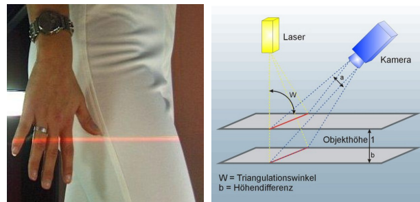
Figure 1. Left: laser stripe on the human body. Right: triangulation method, different object heights result in different triangulation angles that can be measured by the light sensor (images of Vitronic GmbH).
