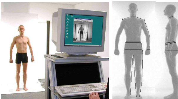
Figure 8. 2D Full body scanner Contour of Human-Solutions. Left: scanning equipment. Right: silhouettes images used for the measurement (images of Human-Solutions).
