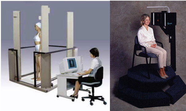
Figure 2. Laser scanning systems. Left: full body scanner BodyLine of Hamamatsu. Right: head scanner Head & Face 3030 3D Color Scanner of Cyberware.
