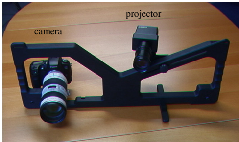
Figure 6. Scanning systems with projection of light: Shapesnatcher of Eyetronics (camera and projector).
