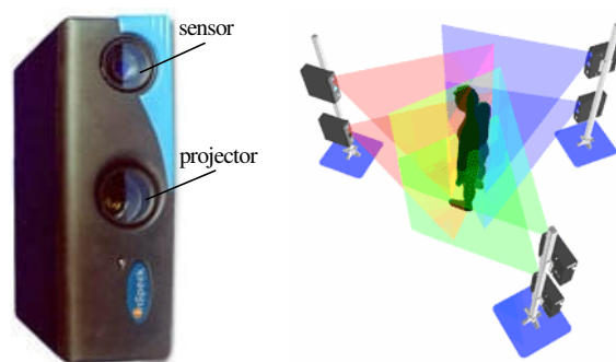
Figure 5. Left: scanning device Capturor of InSpeck. Right: six Capturors compose a full body scanning system (images of InSpeck).
